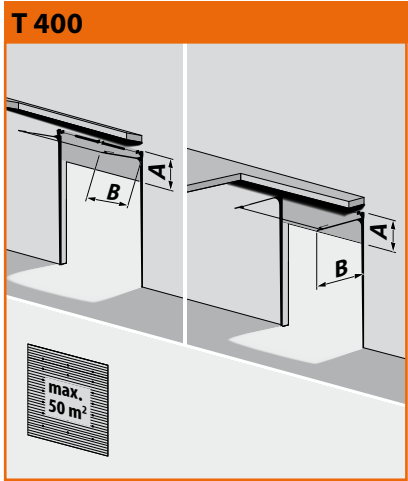
Elevated rail system A= hoisting + 400 mm, B= open height – hoisting + 600 mm
