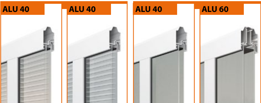
ALU 40 ALU 40 ALU 40 ALU 60 5-core polycarbonate hollow-core plate (20 mm) transparent (light transmittance 63%) 5-core polycarbonate hollow-core plate (20 mm) grey (light transmittance 42%) Double-glazed partially transparent plate (20 mm) in: structural glass (SAN) (light transmittance 80%) Double-glazed partially transparent plate (40 mm) in: structural glass (SAN) (light transmittance 80%)
