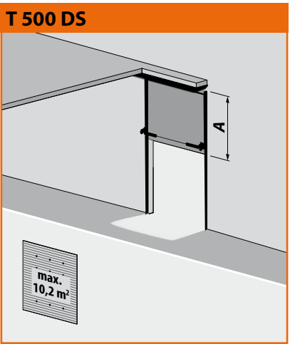
Vertical rail system with low spring axis A= open height + 400 mm Width max. 3,200 mm Height max. 3,200 mm
