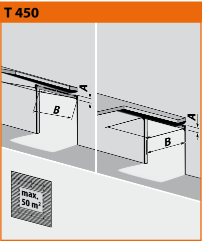
Standard rail system (comes standard) A = 430-510 mm B= open height + 650 mm
