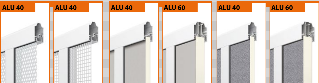
ALU 40 ALU 40 ALU 40 ALU 60 ALU 40 ALU 60 Single-walled perforated ALU plate (2 mm) round perforation (air transmittance 40%) Single-walled perforated ALU plate (2 mm) square perforation (air transmittance 70%) Double-wall closed sandwich version (20 mm), smooth plate on the outside and plaster on the inside Double-wall closed sandwich version (40 mm), smooth plate on the outside and plaster on the inside Double-wall closed sandwich version (20 mm), plaster on the inside and outside Double-wall closed sandwich version (40 mm), plaster on the inside and outside
