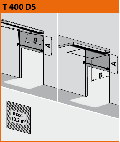
Elevated rail system with low spring axis A= hoisting + 200 mm B= open height – hoisting + 600 mm Width max. 3,200 mm Height max. 3,200 mm Lift min. 1,700 mm
