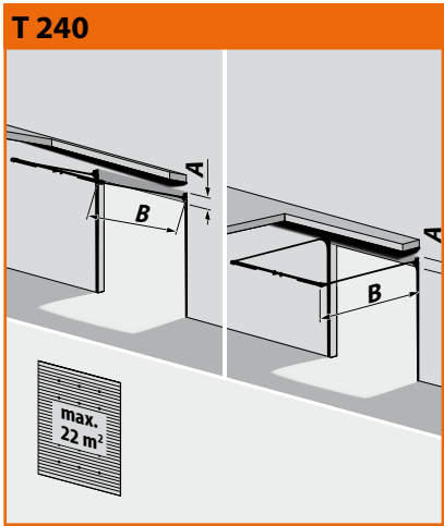
Low built-in rail system, incorporated cables + steel support profile A= 240 mm B= open height + 1,000 mm Width max. 6,500 mm
